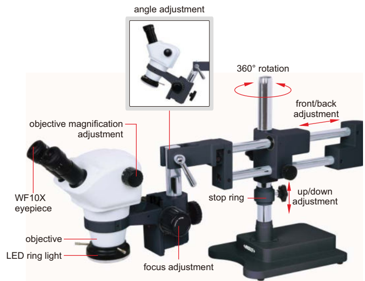
5106-M50 (with stand type B)
